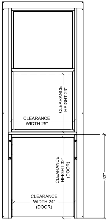
FRONT VIEW
